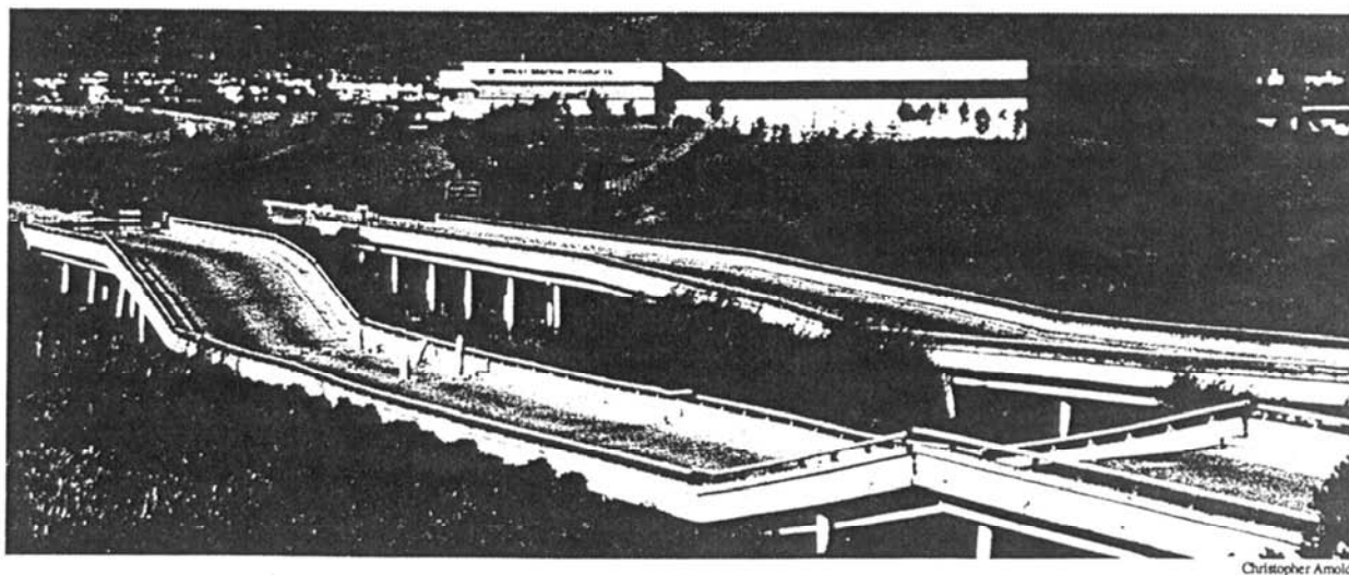
Figure 2.4: Ground failure occurred at this highway, overstressing column/slab connections.
